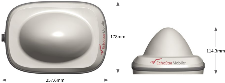
Hughes 4500, Available with vehicle mount, pole mount, and mag mount accessories
